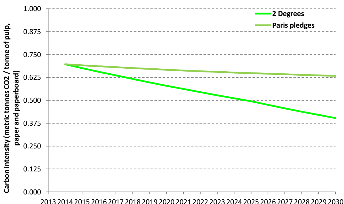
Figure 1 Benchmark global carbon intensity paths for the paper sector (tonnes of CO 2 per tonne of pulp, paper and paperboard) consistent with limiting warming to 2°C and with the sum of the Paris Pledges
