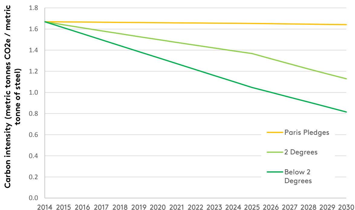
Figure 1 Benchmark global carbon intensity paths for the steel sector
